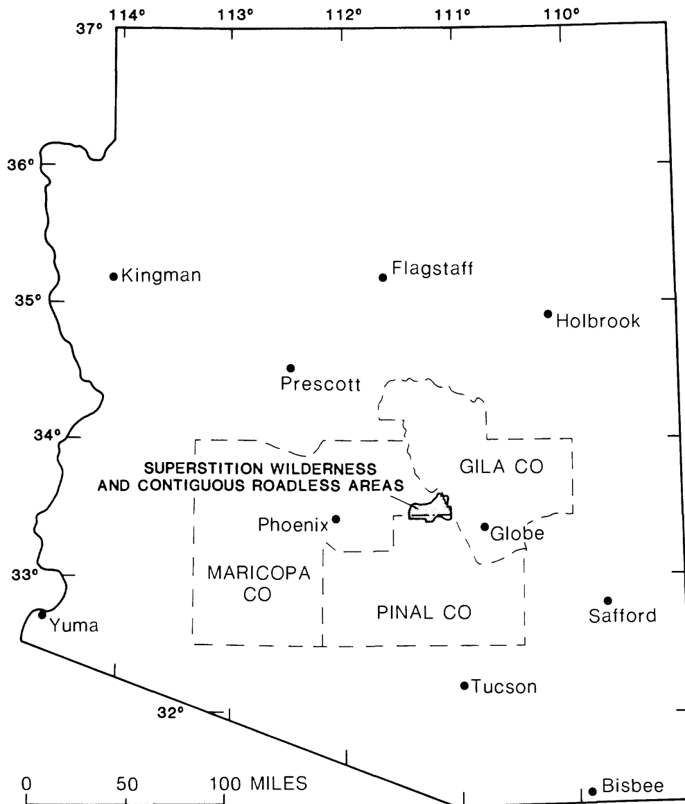
Figure 1.--Index map of Arizona showing approximate location of Superstition Wilderness and contiguous roadless areas.
