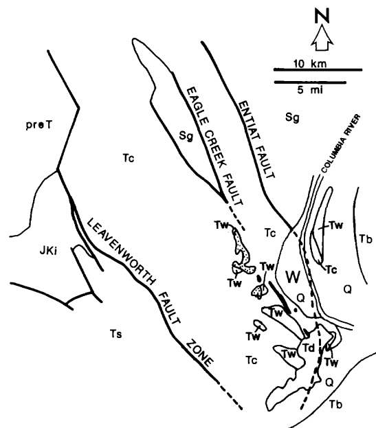
FIG. 1. Generalized geologic map of the Wenatchee region modified from Gresens (1983) and Tabor et al. (1982, 1987). Pre-Tertiary units: JKi, Ingalls tectonic complex; preT, undifferentiated metamorphic and plutonic rocks; Sg, Swakane Biotite Gneiss. Q, Quaternary Tertiary units; Tb, Columbia River Basalt; Tc, Chumstick Formation; Td, Pliocene diamictite; Ts, Swauk Formation; Tw, Wenatchee Formation. Tertiary intrusive rocks: solid black, Eocene; stippled, Oligocene. W = city of Wenatchee.
